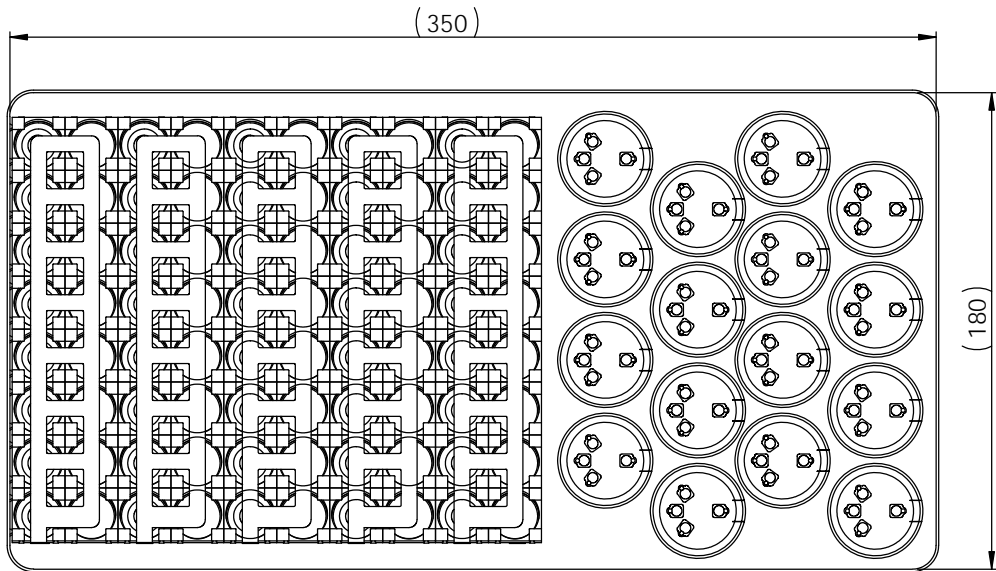
Scooter Battery Box
