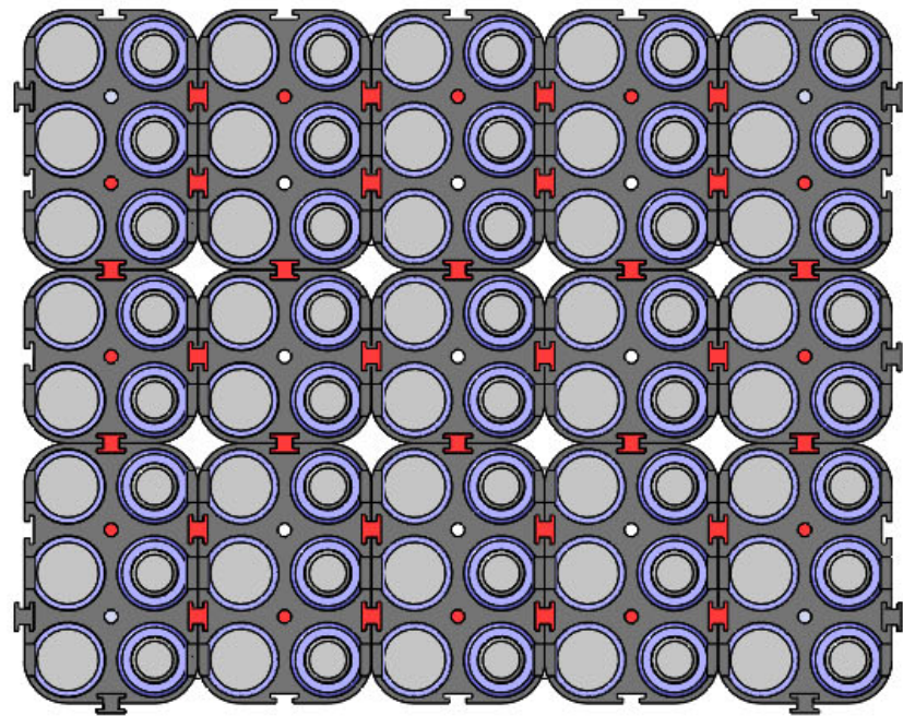
BOTTOM VIEW (WITHOUT ANY BAR)
